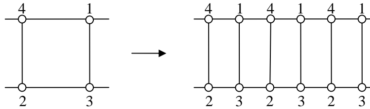
Figure 7: Extending the colouring of a prism
