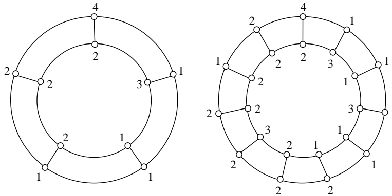
Figure 8: Strong parity vertex colouring of the graphs D_5 and D_{11}
