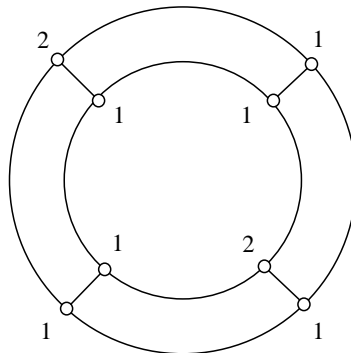
Figure 2: Strong parity vertex colouring of the cube Q
