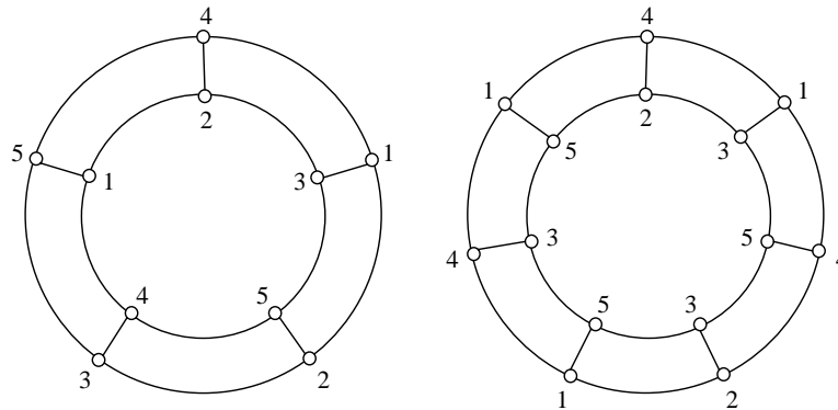
Figure 11: Proper strong parity vertex colouring of the graphs D_5 and D_7
