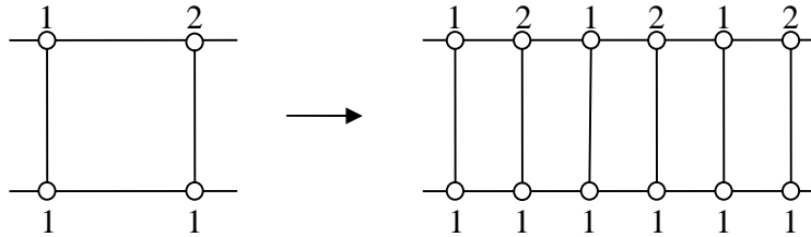
Figure 5: Extending the colouring of a prism
