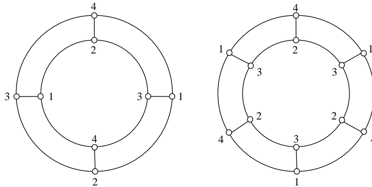
Figure 10: Proper strong parity vertex colouring of the graphs D_4 and D_6
